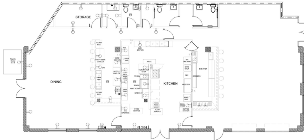
ELECTRICAL PLAN Scale: 1'-0" = 3/16"
