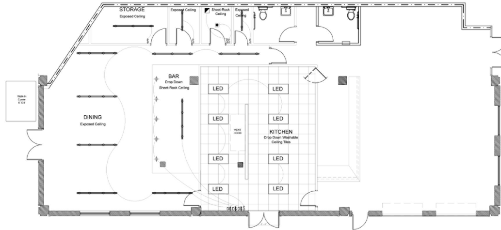
REFLECTIVE CEILING PLAN Scale: 1'-0" = 3/16"
