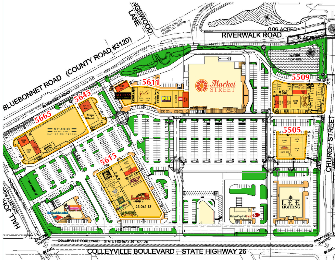
01 SITE PLAN SCALE: 1" = 50'-0" DATE: 10/10/2016
